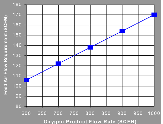
AirSep "AS-K" Oxygen Generator Feed Air Requirement (93% nominal oxygen)
